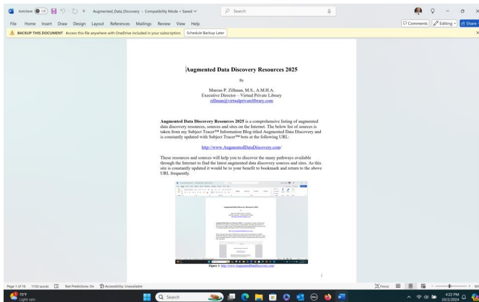
Figure 1: http://www.AugmentedDataDiscovery.com/
