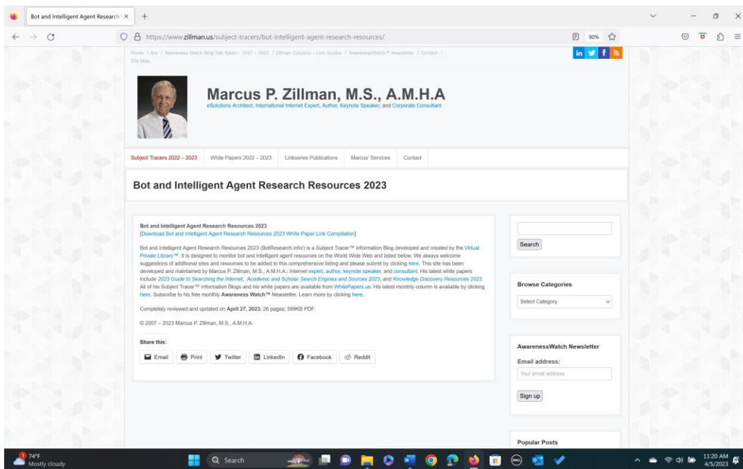
Figure 1: Bot Research 2023
