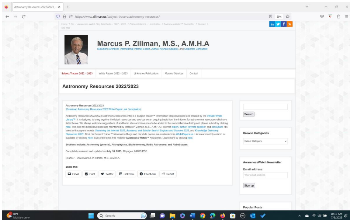
Figure 1: Astronomy Resources 2023
